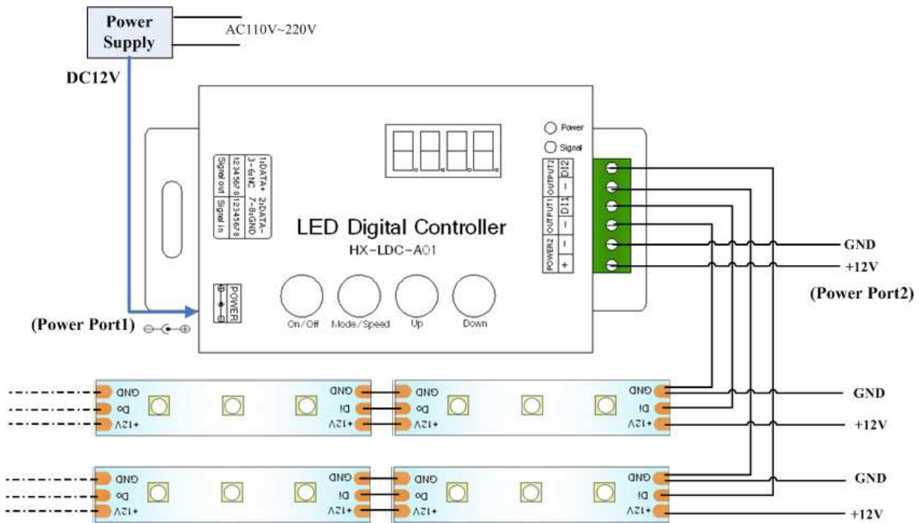
Application Circuit2, (Each controller can be individually powered, can also share power)
