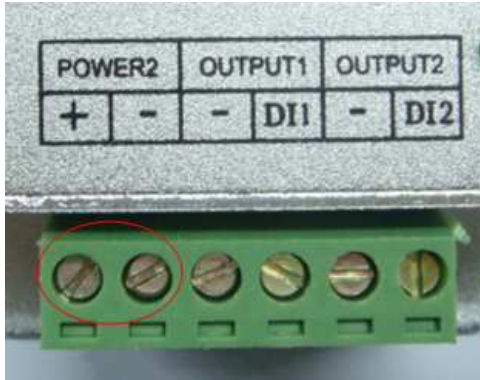
Adopt male and female connector with screw.
