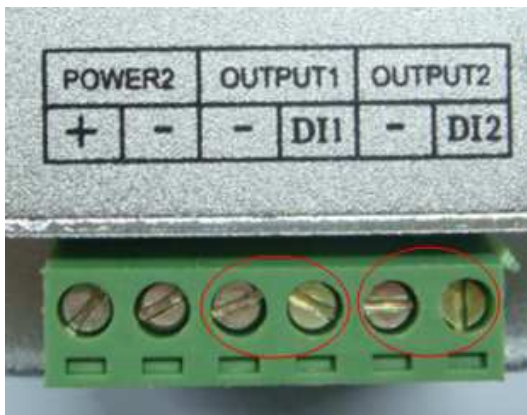
Adopt male and female connector with screw.
